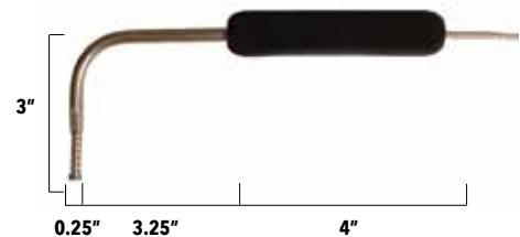
90° Rugged (SR90-)
