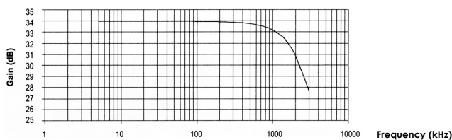
Figure 1: Small Signal Frequency Response (Typical) Amplifier Gain measured with 900 mV peak-to-peak input. Amplifier Frequency Response (-3 dB) at 2 MHz.
