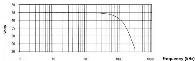
Figure 2: Small Signal Frequency Response (Typical) Amplifier Gain measured with 900 mV peak-to-peak input. Same as Figure 1 but Y-axis is Volts instead of dB.
